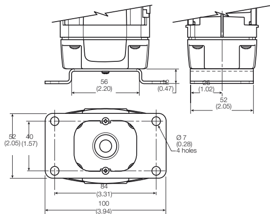
Foot Bracket
