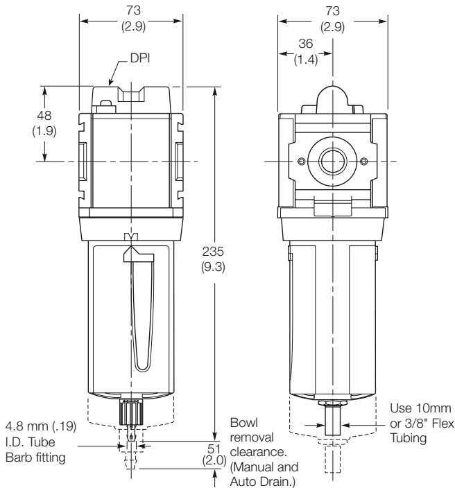
Manual Drain
