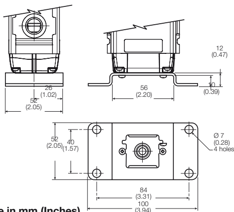
Foot Bracket
