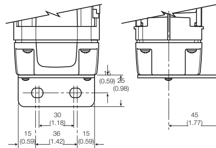
Foot Bracket
