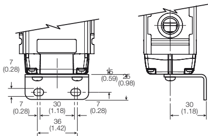
Foot Bracket
